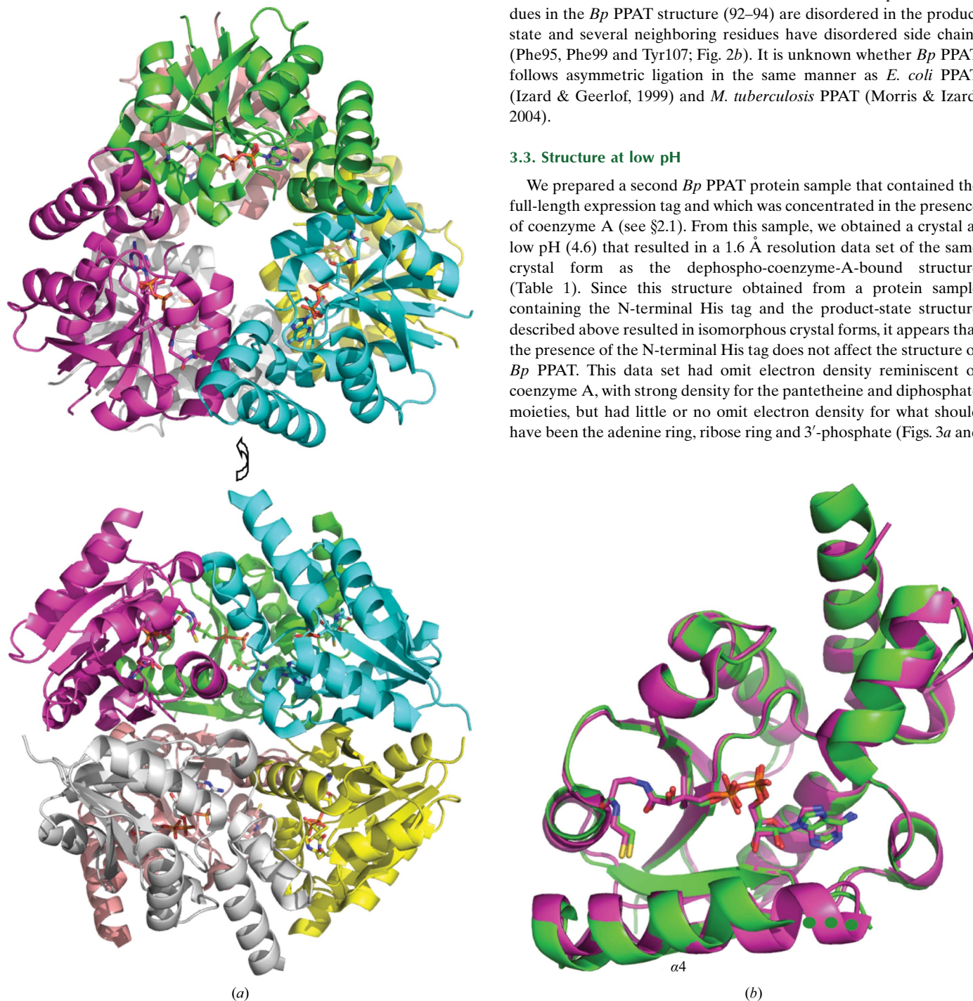
Figure 2 Crystal structure of Bp PPAT solved at 2.1 \text{\AA} resolution. ( a ) Biologically relevant hexameric structure of Bp PPAT from a crystal structure with bound dephospho-coenzyme A solved at 2.1 \text{\AA} resolution. ( b ) Overlay of the dephospho-coenzyme A-bound structures of Bp PPAT (green) and E. coli PPAT (PDB entry 1b6t, magenta; Izard & Geerlof, 1999). Green spheres are used to illustrate disordered residues in the Bp PPAT crystal structures. Figs. 2 and 3 were prepared using PyMOL (DeLano, 2002).
